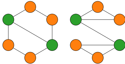
(b) 1-WL after one iteration.
