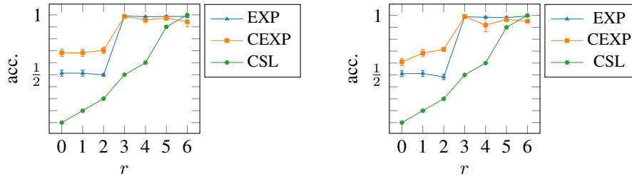
Figure 4: Test accuracy on synthetic classification task: (left) shared and (right) non-shared weights.
