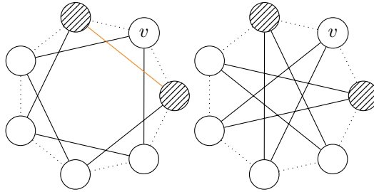
(c) CSL example, skip length 2 (left) and 3 (right).
