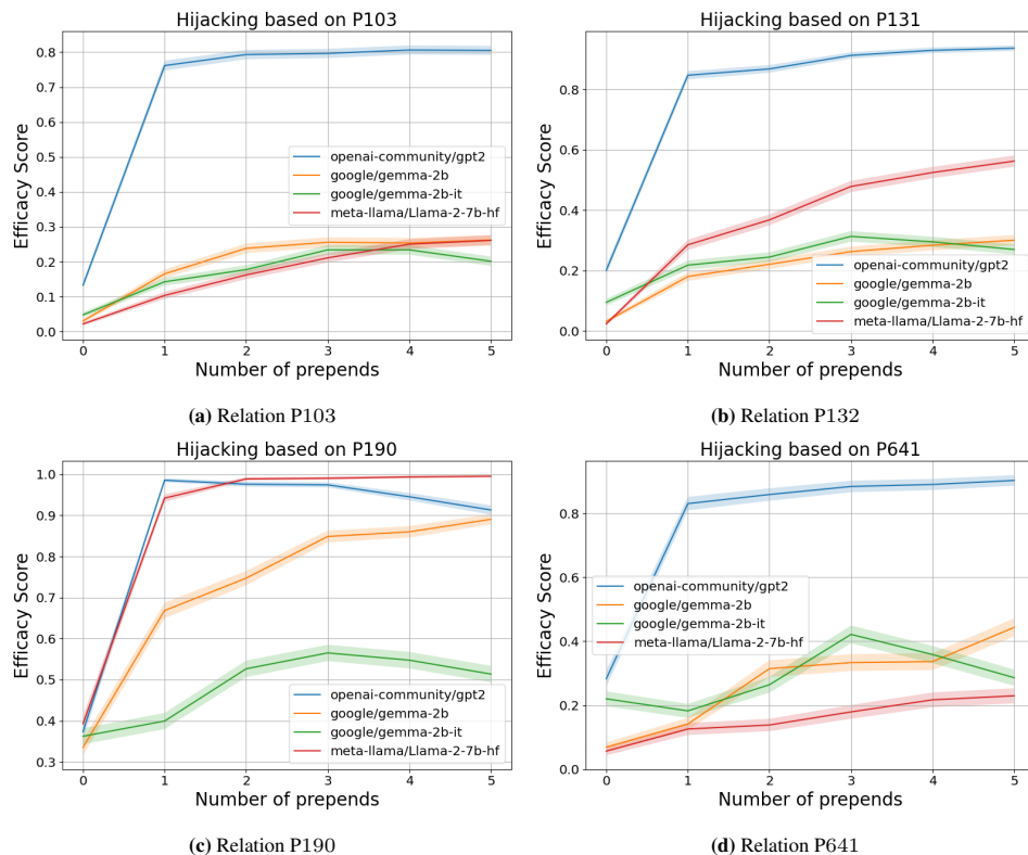
Figure C.2: Context hijacking based on relation IDs can result in LLMs output incorrect tokens. This figure shows efficacy score versus the number of preponds for various LLMs on the COUNTERFACT dataset with hijacking scheme presented in Table 2.
