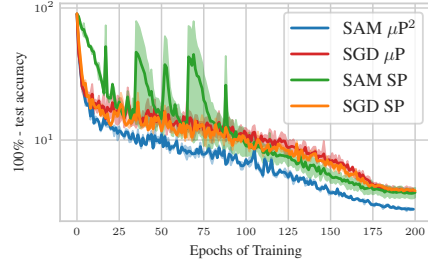
Figure 5: ( Stable training dynamics ) SAM in \mu\mathbf{P}^2 stabilizes training dynamics for a ResNet-18 with width multiplier 2.
