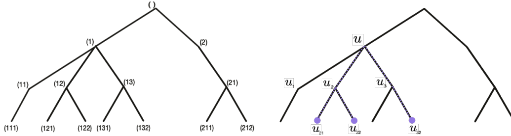
Figure 2: In the these figures, we present the vertices as words and adapt the notations u_1, u_2, \dots , for the descendants of u . For the right figure, if S = \{u_{21}, u_{22}, u_{32}\} , then \rho(S) = u , I(S) = \{2, 3\} , and S_2 = \{u_{21}, u_{22}\} , S_3 = \{u_{32}\} . Further, S_1 \in \mathcal{A}_3 , S_2 \in \mathcal{A}_2 , and S_3 \in \mathcal{A}_1 .
