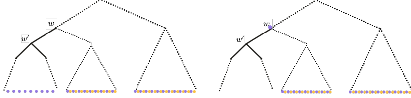
Figure 3: In the left figure, the purple dots represent the corresponding input variables for f_\alpha , and the yellow dots represent the corresponding input variables for f_\beta . In the right figure, the purple dots represent the corresponding input variables for \mathbb{E}[f_\alpha(X) | X_{\underline{z}w_1}] and the variables do not involve x_v for vertex v not illustrated due to the Markov property.
