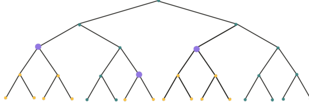
Figure 5: In this figure, the purple dots represent the set U . The yellow dots represent the vertices corresponding to the variables x_{<U} , and the green dots represent the vertices corresponding to the variables x_{\not\leq U} .
