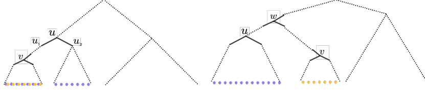
Figure 4: In both figures, the purple dots represent the corresponding input variables for f_u , and the yellow dots represent the corresponding input variables for f_v . In the left figure, we have v \leq u_1 < u . In the right figure, we have u and v are incomparable and w is the nearest common ancestor.
