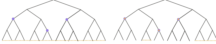
Figure 6: The purple dots represent the set U . In the left figure, the yellow dots represent the vertices corresponding to the variables of f . In the right figure, the yellow dots represent the vertices corresponding to the variable of \mathbb{E}_U f .
