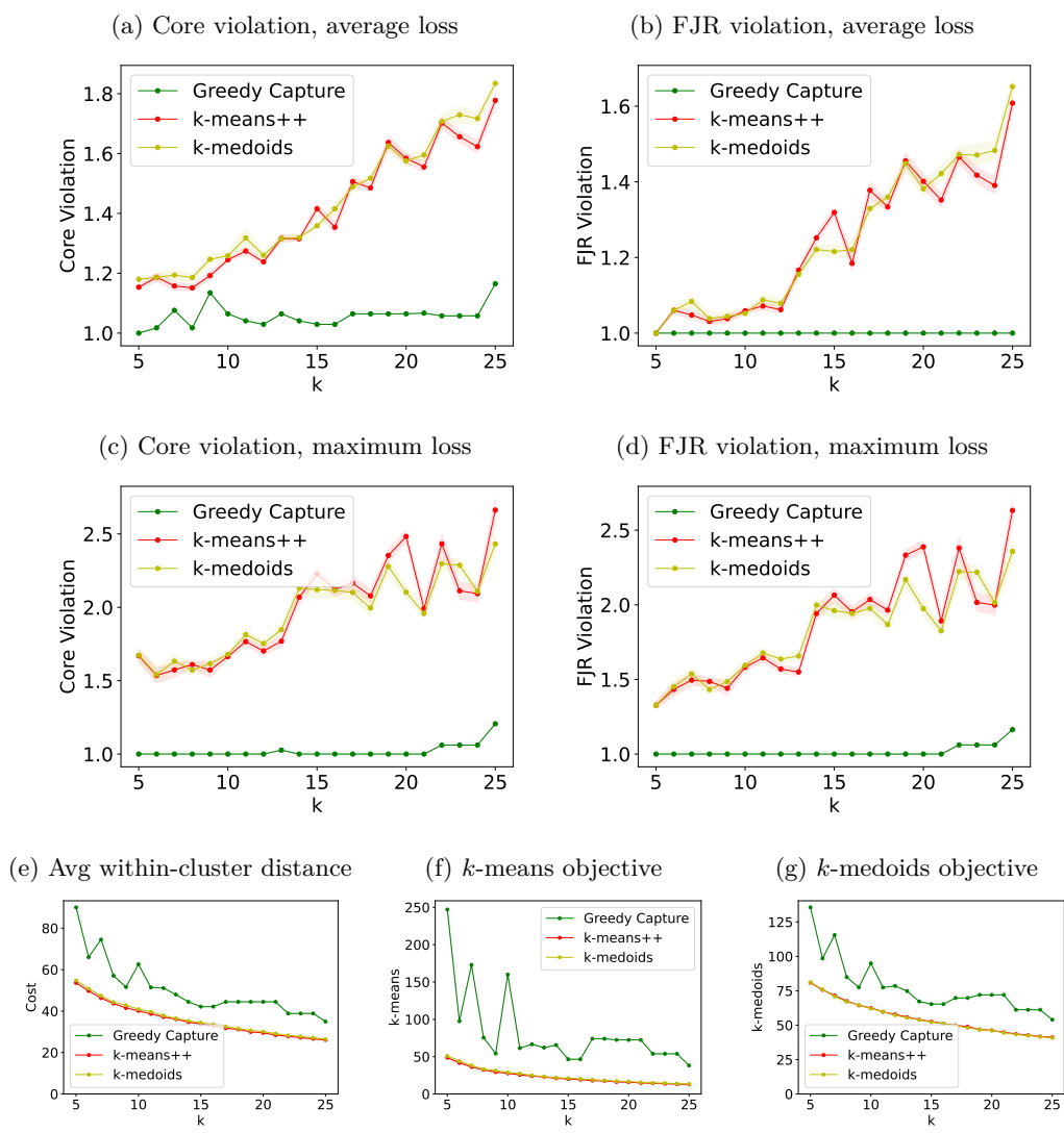
Figure 5: Iris dataset
