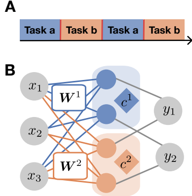
Figure 1: The open-ended learning setting and the modeling approach. A. Example of the blocked curriculum with two tasks. B. Neural Task Abstraction (NTA) model updates \mathbf{W}^p through gradient descent, but also the gating variables c^p , leading to task abstractions emerging in the gating layer.
