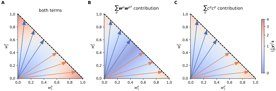
Figure A.8: Specialized students and gates accelerate adaptation. Heatmaps of the dot product (\frac{d}{dt} \mathbf{y})^T \boldsymbol{\varepsilon} contributions for different terms of the Neural Tangent Kernel (NTK), depending on specialization of weight vectors \mathbf{w}^1 (blue), \mathbf{w}^2 (orange), of which three pairs corresponding to different degrees of specialization are shown here (pairs are formed by vectors that are symmetric along the diagonal). c^1, c^2 are scaled so that the sum lies on the dashed black line (given by L^1 regularization). A. shows the total contribution of both terms of Eq. (20) combined, B. isolates the contribution from the \mathbf{w}^p \mathbf{w}^{pT} term, and C. displays the contribution from the c^p c^p term. Dashed lines indicate possible solutions.
