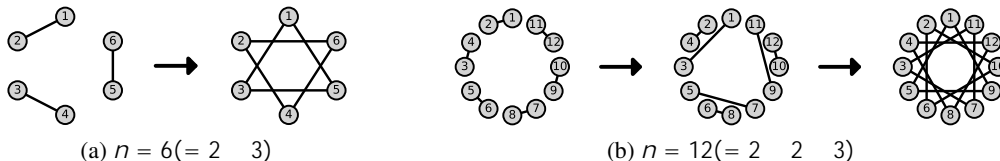
Figure 2: Illustration of the 2-PEER HYPER-HYPERCUBE GRAPH.
