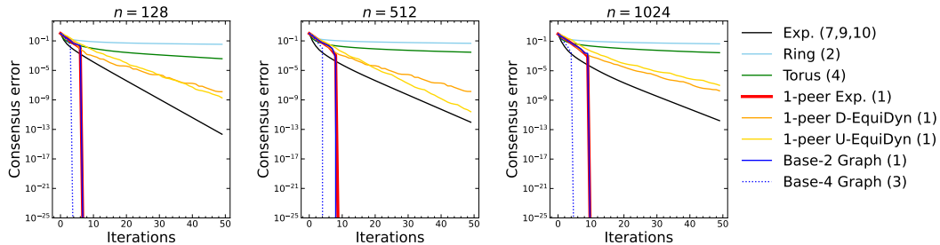
Figure 21: Comparison of consensus rates among different topologies when the number of nodes n is a power of 2. Because the BASE- f3, 5g GRAPH are the same as the BASE- f2, 4g GRAPH, respectively, when n is a power of 2, we omit the results of the BASE- f3, 5g GRAPH.
