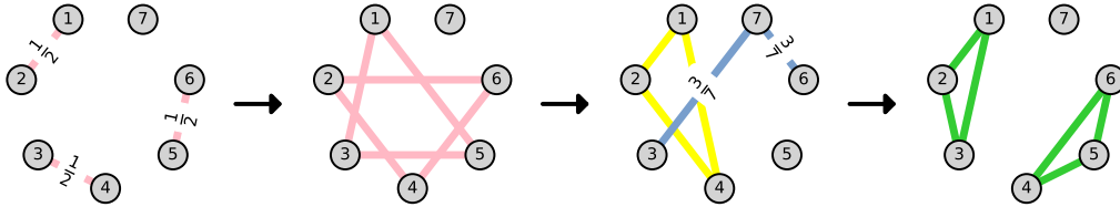
Figure 11: k = 2, n = 7 (= 2 \cdot 3 + 1) . The value on the edge indicates the edge weight. For simplicity, we omit the edge value when it is \frac{1}{3} .
