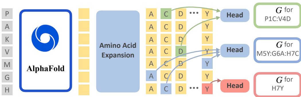
Figure 3: Mutate Everything decodes many mutations. Each token output by the backbone x_j is expanded to 20 tokens z(\mu) , each corresponding to one unique amino acid type (yellow with amino acid types). For each mutation set M , we first aggregate the features corresponding to each mutation’s position and amino acid being mutated to (arrows). A lightweight head g then decodes the aggregated features to obtain the predicted \Delta\Delta G . These heads are illustrated in Figure 2b and Figure 2c. Parallel feature aggregation and decoding enable efficient stability prediction for millions of mutations.
