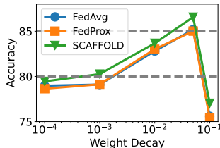
Figure 1: Accuracy of three FL algorithms (i.e., FedAvg, FedProx, and SCAFFOLD) after 1000 rounds using different weight decay coefficients. See details in Section 3
