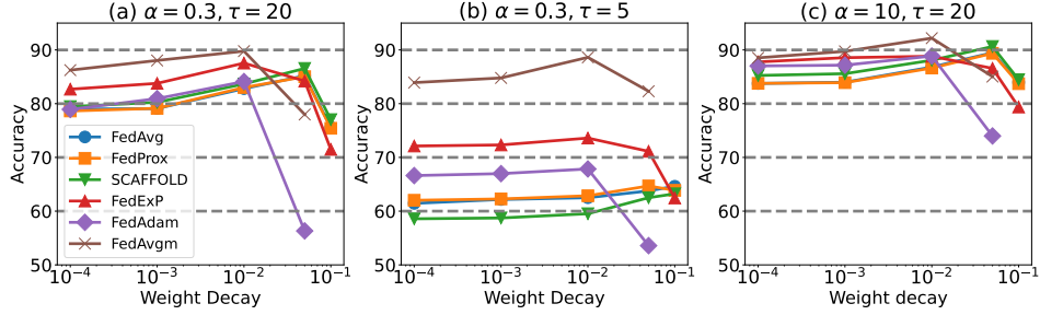
Figure 2: Influence of weight decay for different settings. We train each algorithm ( i.e. , FedAvg, FedProx, SCAFFOLD, FedExp, FedAdam, FedAvgm) over 1000 rounds with \tau local steps per round, a local learning rate of 0.01, and a global learning rate of 1.0. We apply a decay for the local learning rate of 0.998 per round and a gradient clipping of max norm 10 as per [24]. Given that multiple local steps and imbalanced data distribution are two distinguishing features of FL, we utilize various pairs of (\alpha, \tau) to observe their influence on the results. The baseline setting is chosen to be (\alpha, \tau) = (0.3, 20) , resulting in a highly imbalanced data distribution. The second configuration reduces the number of local updates to (\alpha, \tau) = (0.3, 5) . The third configuration employs a balanced data distribution with (\alpha, \tau) = (10, 20) .
