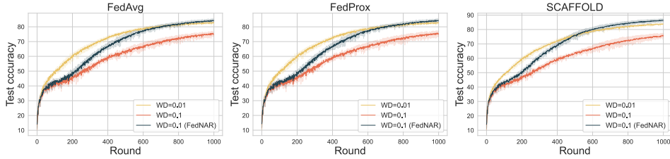
Figure 4: The self-adjusting capability of FedNAR. WD denotes the initial weight decay value applied in the first round. It is crucial to note that in each round t , the weight decay remains consistent for both the baseline methods and FedNAR. The distinction lies in FedNAR’s adoption of co-clipping across both weight decay and gradient. We drew comparisons among FedAvg, FedProx, and SCAFFOLD with WD values of 0.1 and 0.01. The utilization of 0.1 as the WD value proved to be less than ideal, resulting in a performance decrement in the baseline methods. Conversely, FedNAR initially mimics this trend but swiftly ameliorates during the subsequent stages, outstripping the baselines even with a more favorable initial WD value of 0.01.
