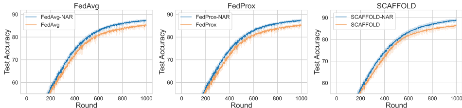
Figure 3: Test accuracy curve for FedAvg, FedProx, SCAFFOLD and their FedNAR variants for \alpha = 0.3 . For each training, we take 3 random seeds.
