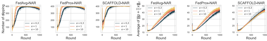
Figure 5: Frequency and strength of clipping. In every round, there is a sum total of 20 clients, and each client carries out 20 updates, leading to a collective tally of 400 updates per round. We monitor the count of clipping instances within these 400 updates during each round and compute the average norm of the updates subjected to clipping. We execute experiments for diverse \alpha values, and for every algorithm, we present the outcomes utilizing three distinct seeds.
