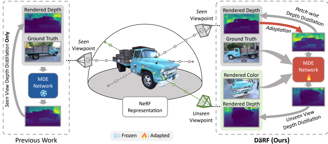
Figure 1: Overview. DäRF shows robust optimization of few-shot NeRF through MDE’s geometric prior, removing inherent ambiguity from MDE through novel patch-wise distillation loss and MDE adaptation. Unlike existing work [45] that distills depths by applying pretrained MDE to NeRF at seen view only, our DäRF fully exploits the ability of MDE by jointly optimizing NeRF and MDE at a specific scene, and distilling the monocular depth prior to NeRF at both seen and unseen views.
