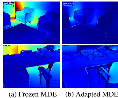
Figure 4: Error map visualization. MDE adaptation results in a reduction of errors.
