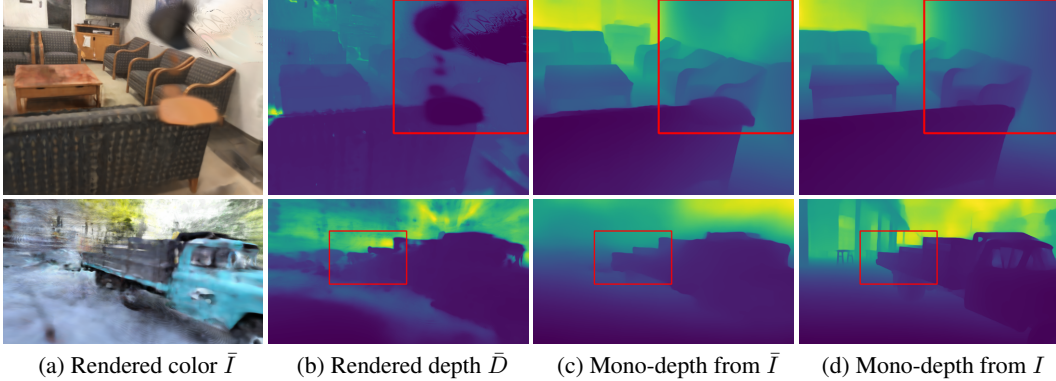
Figure 3: Robustness of MDE model for multi-view scale ambiguity and artifacts: (a-b) color and depth of NeRF rendered in the early stage of the training, (c-d) monocular depths estimated from rendered image \bar{I} and input image I . The results show that MDE model ignores the artifacts of rendered images by NeRF, enabling reliable supervision for seen and unseen viewpoint.
