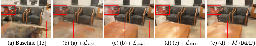
Figure 8: Visualization of ablation studies on ScanNet [10].
