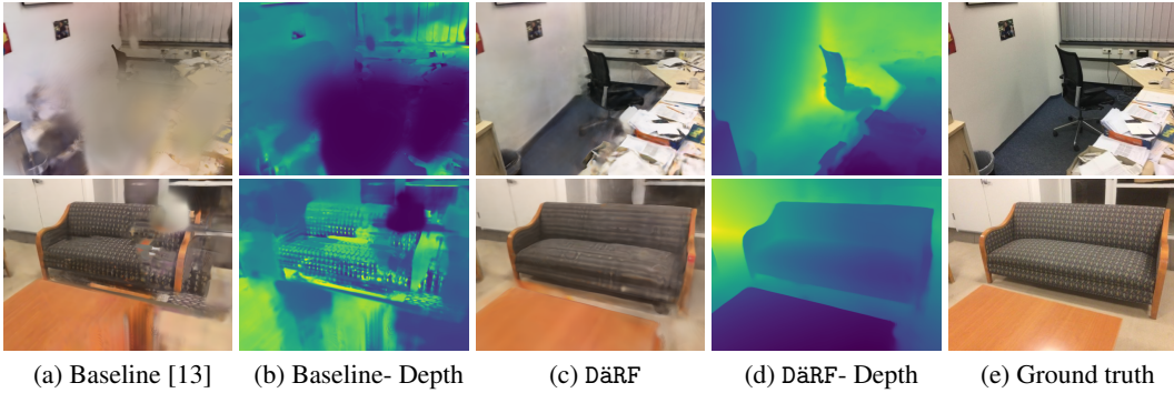
Figure 6: Qualitative results on ScanNet [10] with 9 - 10 input views.
