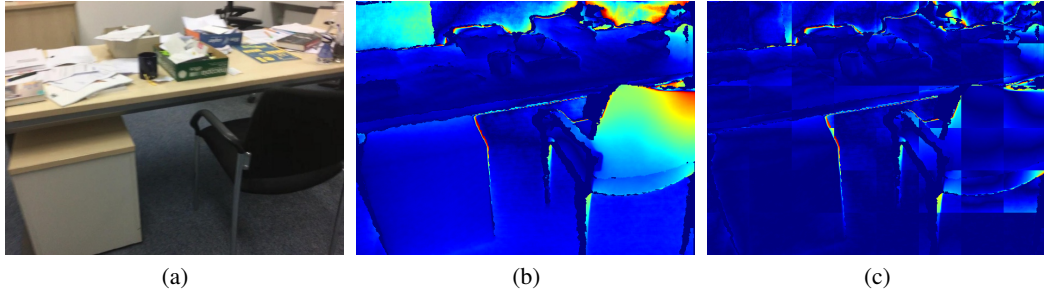
Figure 2: Effectiveness of patch-wise scale and shift adjustment: (a) input image, (b) monocular depth with image-level adjustment, and (c) monocular depth with patch-level adjustment. We visualize the error of adjusted monocular depth from input image compared to GT depth value. The proposed patch-level adjustment helps to minimize the errors caused by inconsistency in depth differences among objects.
