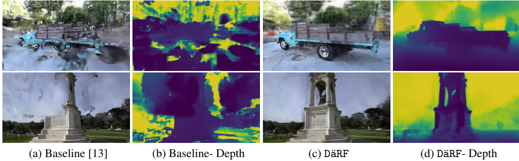
Figure 7: Qualitative results on Tanks and Temples [19].
