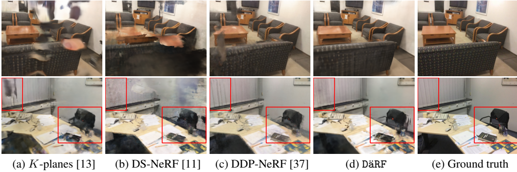
Figure 5: Qualitative results of on ScanNet [10] with 18 - 20 input views.
