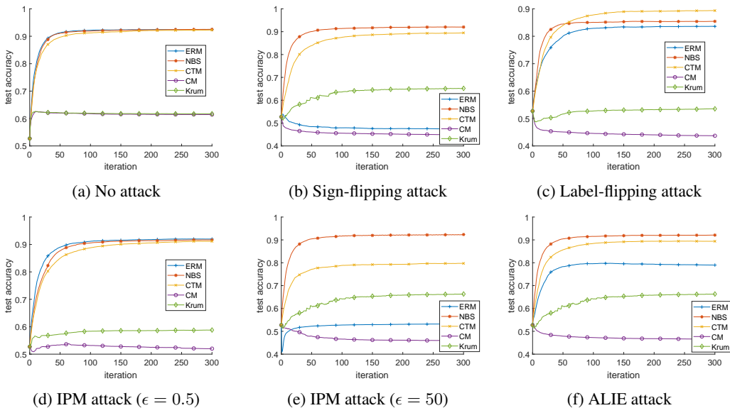
Figure 1: Model accuracy of different robust aggregation schemes under various attacks.
