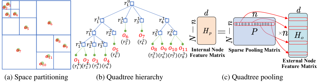
Figure 2: An example of a quadtree and pooling operation.
