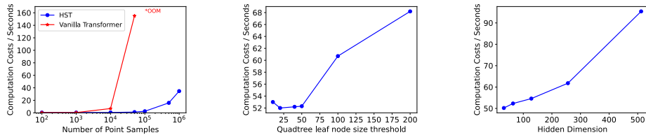
(a) Computation cost per epoch for 64 training samples. (b) Computation cost per epoch versus leaf node size threshold for 5K training samples. (c) Computation cost per epoch versus hidden dimension for 5K training samples.
