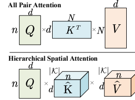
Figure 4: Sparse spatial attention with selective key set.
