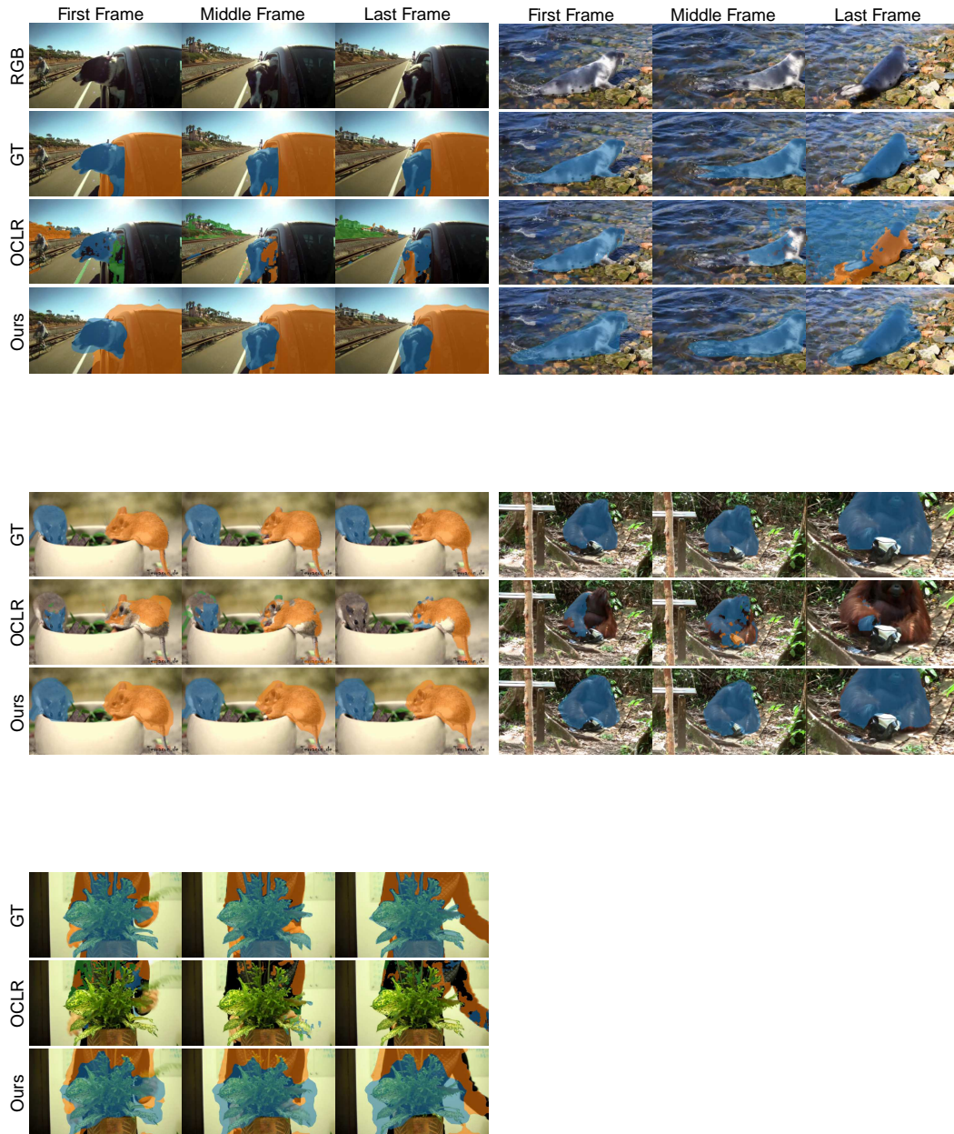
Figure 13: Qualitative results of multi-object video segmentation on YTVIS19 after Hungarian Matching is applied. Segmentation results of OCLR [83] are provided in third row.
