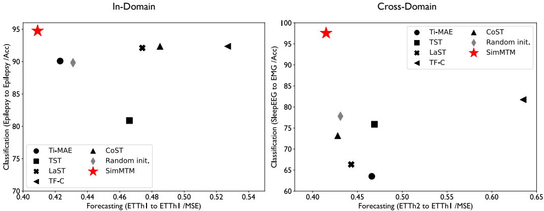
Figure 3: Performance comparison of time series pre-training methods in forecasting ( MSE \downarrow ) and classification ( Acc \uparrow ) tasks, including both in-domain (left) and cross-domain (right) settings.
