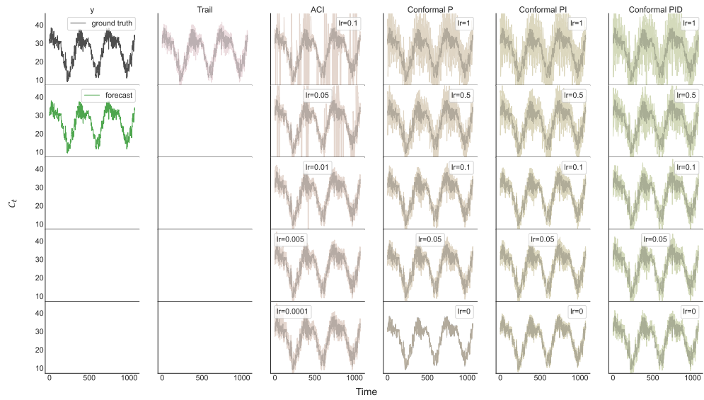
Figure 14: Results for the Delhi temperature data set.
