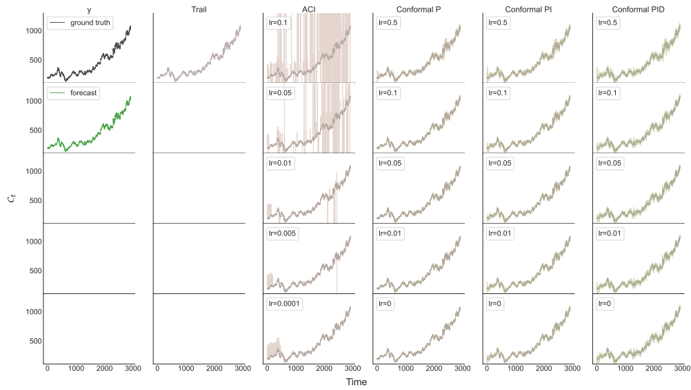
Figure 12: Results for the Google data set.
