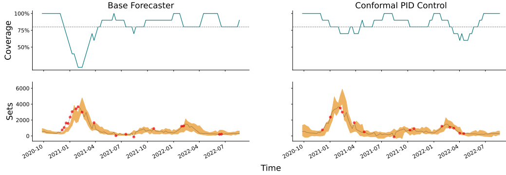
Figure 2: Results for 4-week ahead COVID-19 death forecasting in California. The left column shows the COVID-19 Forecast Hub ensemble model, and the right column shows conformal PID control using the tan integrator, and a scorecaster given by \ell_1 -penalized quantile regression on all past forecasts, cases, and deaths from all 50 states. The top row plots coverage, averaged over a trailing window of 10 weeks. The nominal coverage level is 1 - \alpha = 0.8 and marked by a gray dotted line. The bottom row plots the prediction sets in gold along with the ground-truth times series (death counts). Miscoverage events are indicated by red dots. Summary statistics such as the coverage and average set size are available in Table 1.
