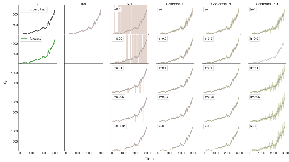
Figure 11: Results for the Amazon data set.
