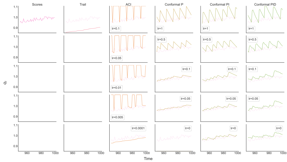
Figure 17: Results for an increasing score sequence.
