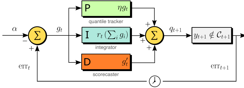
Figure 1: Conformal PID Control, expressed as a block diagram.
