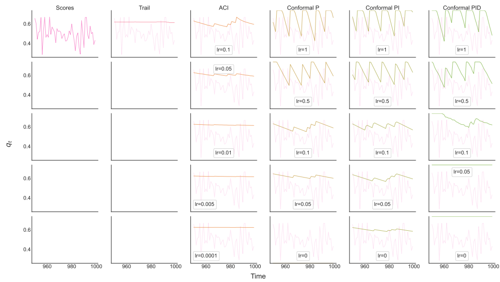
Figure 16: Results for an i.i.d. score sequence.
