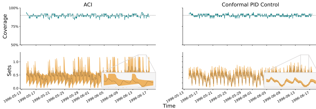
Figure 3: Results for electricity demand forecasting. The left column shows adaptive conformal inference (ACI), and the right column shows conformal PID control. The base forecaster is a Transformer model, and we use a tan integrator and a Theta scorecaster. The format of the figure follows that of Figure 2, except the nominal coverage is now 1 - \alpha = 0.9 , and the coverage is averaged over a trailing window of 50 points (we also omit the red dots which mark miscoverage events). Summary statistics are available in Table 2.
