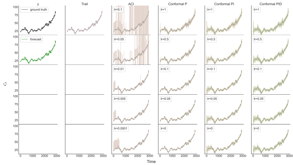
Figure 13: Results for the Microsoft data set.
