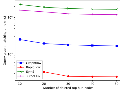
(b) Query time on pattern 3
