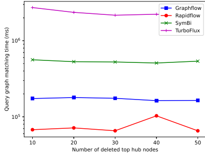
(a) Query time on pattern 1
