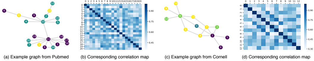
Figure 6: Example graphs and correlation maps. The graphs are randomly sampled from Pubmed and Cornell. The correlation maps are obtained based on the pair-wise similarities of learned posteriors.
