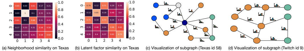
Figure 5: The visualization and case study results (best viewed on a computer screen and note that the latent distribution of each link need to be zoomed in to be better visible).
