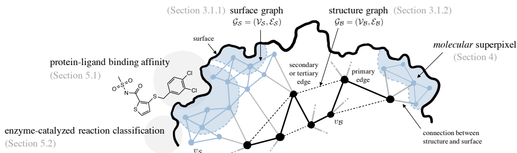
Figure 1: Overview of HOLOPROT Our multi-scale protein representation algorithm integrates primary, secondary and tertiary elements of protein structures and connects them to the surface. We extract higher-level protein motifs by introducing molecular superpixels. Both structure and surface are represented as graphs \mathcal{G}_B and \mathcal{G}_S , respectively. The method is evaluated on two representative tasks, protein-ligand binding affinity and enzyme-catalyzed reaction classification.
