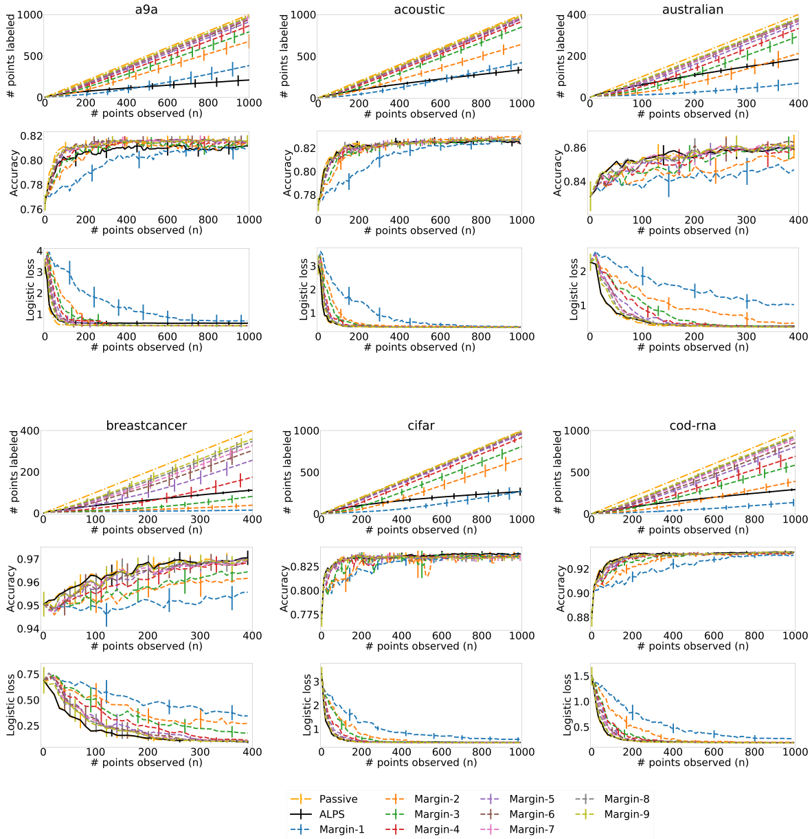
Figure 12: Comparison of all nine margin algorithms to passive learning and ALPS for 4-layer networks (1/3). The margin algorithms are ordered from the smallest to the largest threshold in \Gamma_m , where Margin-1 corresponds to the smallest threshold, Margin-2 to the second smallest, etc. The figures shows the mean over the 50 trials and twice its standard error of the number of labeled points, accuracy and logistic loss on the test set of the model returned by each algorithm as a function of the number of observed points (or rounds) n .
