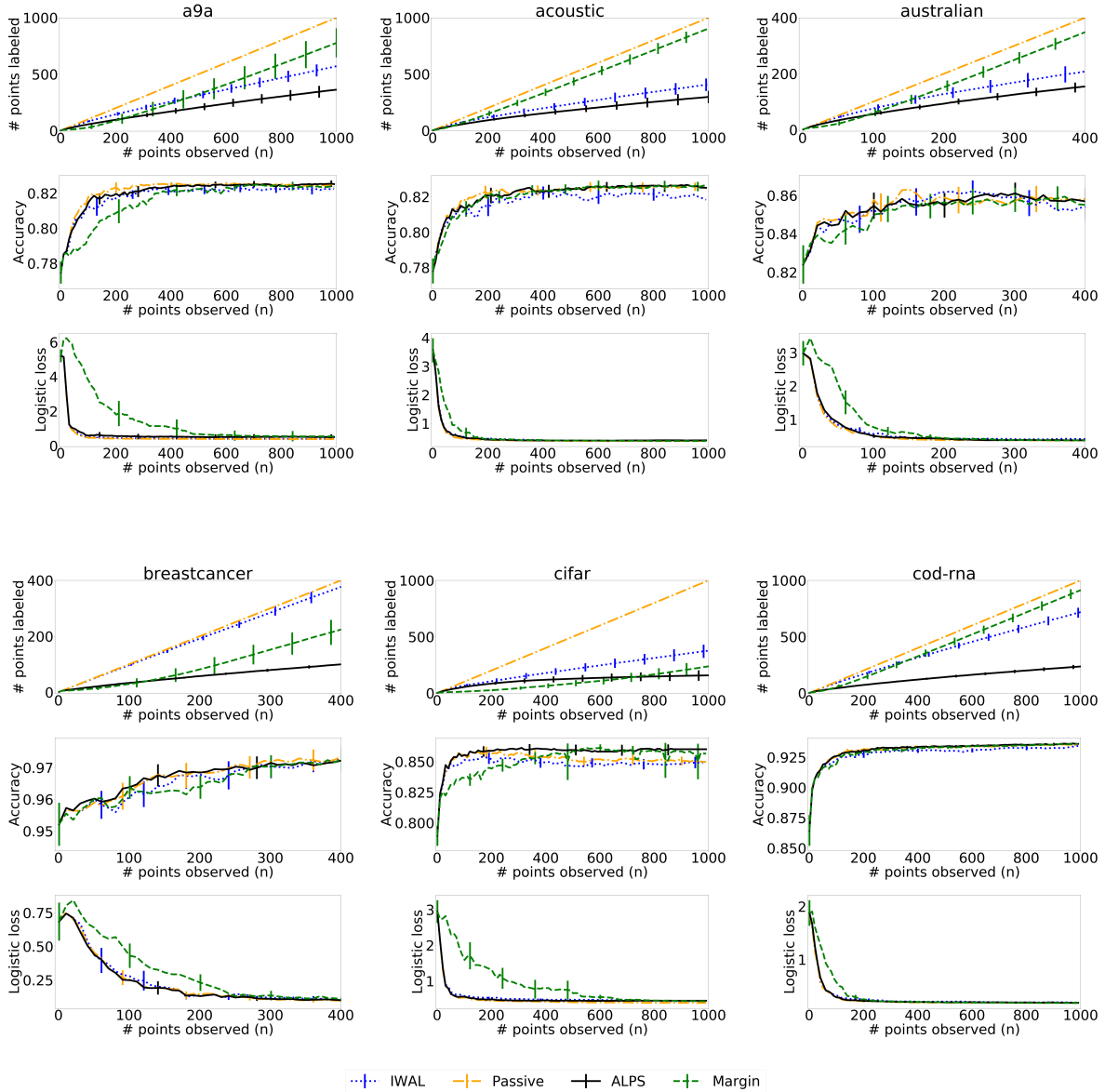
Figure 3: Comparison of the ALPS algorithm, the IWAL algorithm, the ex-post best margin algorithm and the passive learning algorithm for 3-layer networks (1/3). The figures shows the mean over the 50 trials and twice its standard error of the number of labeled points, accuracy and logistic loss on the test set of the model returned by each algorithm as a function of the number of observed points (or rounds) n .
