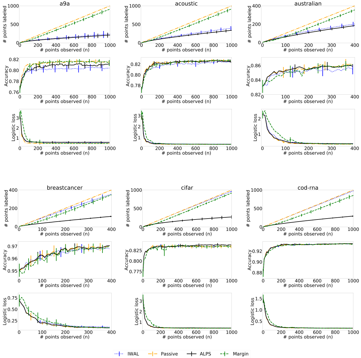
Figure 9: Comparison of the ALPS algorithm, the IWAL algorithm, the ex-post best margin algorithm and the passive learning algorithm for 4-layer networks (1/3). The figures shows the mean over the 50 trials and twice its standard error of the number of labeled points, accuracy and logistic loss on the test set of the model returned by each algorithm as a function of the number of observed points (or rounds) n .
