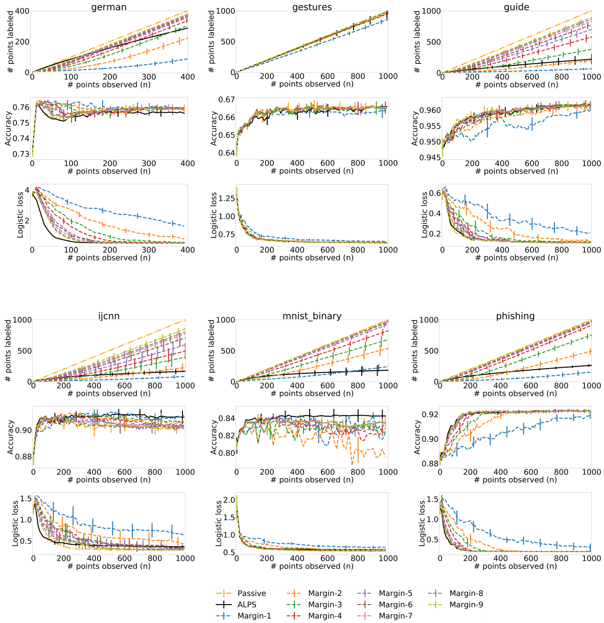
Figure 13: Comparison of all nine margin algorithms to passive learning and ALPS for 4-layer networks (2/3). The margin algorithms are ordered from the smallest to the largest threshold in \Gamma_m , where Margin-1 corresponds to the smallest threshold, Margin-2 to the second smallest, etc. The figures shows the mean over the 50 trials and twice its standard error of the number of labeled points, accuracy and logistic loss on the test set of the model returned by each algorithm as a function of the number of observed points (or rounds) n .
