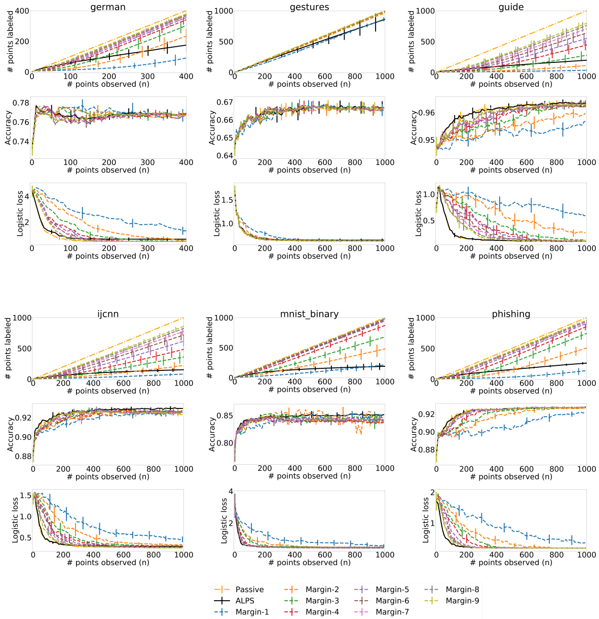
Figure 7: Comparison of all nine margin algorithms to passive learning and ALPS for 3-layer networks (2/3). The margin algorithms are ordered from the smallest to the largest threshold in \Gamma_m , where Margin-1 corresponds to the smallest threshold, Margin-2 to the second smallest, etc. The figures shows the mean over the 50 trials and twice its standard error of the number of labeled points, accuracy and logistic loss on the test set of the model returned by each algorithm as a function of the number of observed points (or rounds) n .
