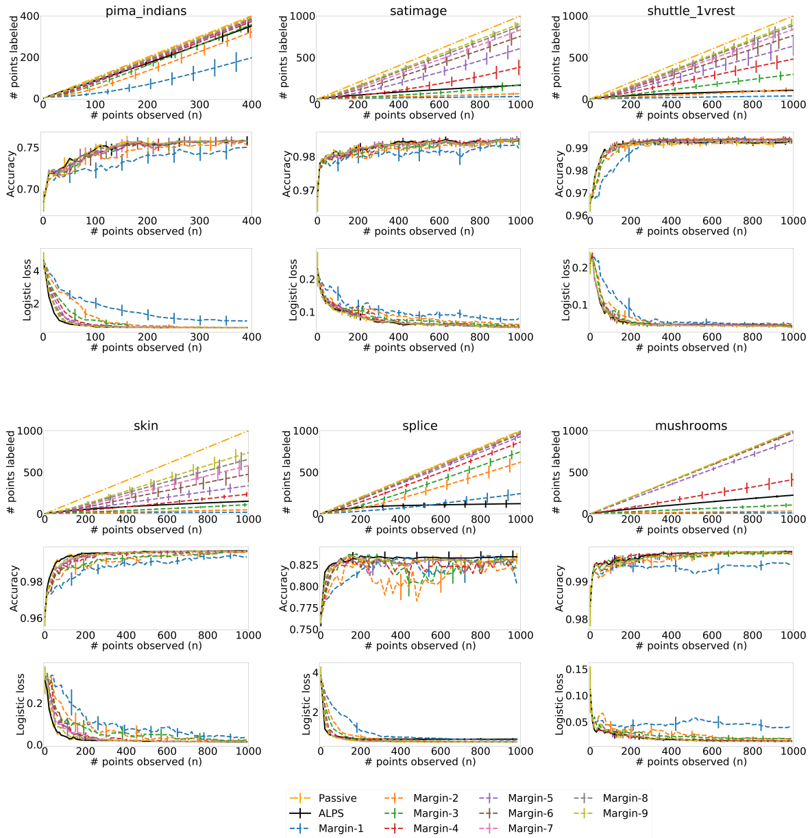
Figure 14: Comparison of all nine margin algorithms to passive learning and ALPS for 4-layer networks (3/3). The margin algorithms are ordered from the smallest to the largest threshold in \Gamma_m , where Margin-1 corresponds to the smallest threshold, Margin-2 to the second smallest, etc. The figures shows the mean over the 50 trials and twice its standard error of the number of labeled points, accuracy and logistic loss on the test set of the model returned by each algorithm as a function of the number of observed points (or rounds) n .
