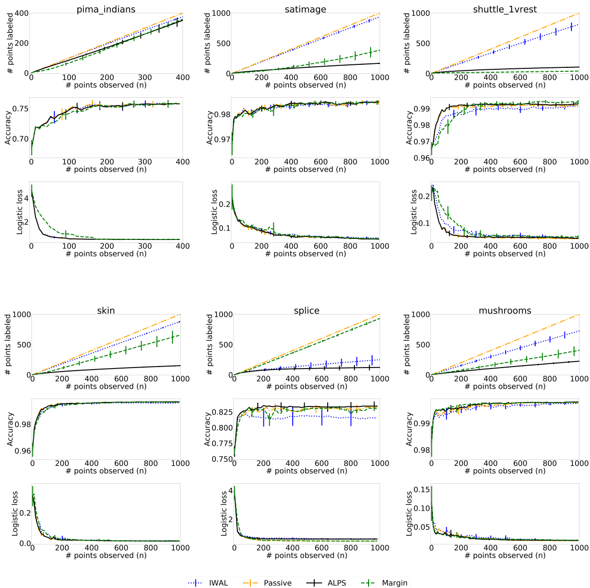
Figure 11: Comparison of the ALPS algorithm, the IWAL algorithm, the ex-post best margin algorithm and the passive learning algorithm for 4-layer networks (3/3). The figures shows the mean over the 50 trials and twice its standard error of the number of labeled points, accuracy and logistic loss on the test set of the model returned by each algorithm as a function of the number of observed points (or rounds) n .
