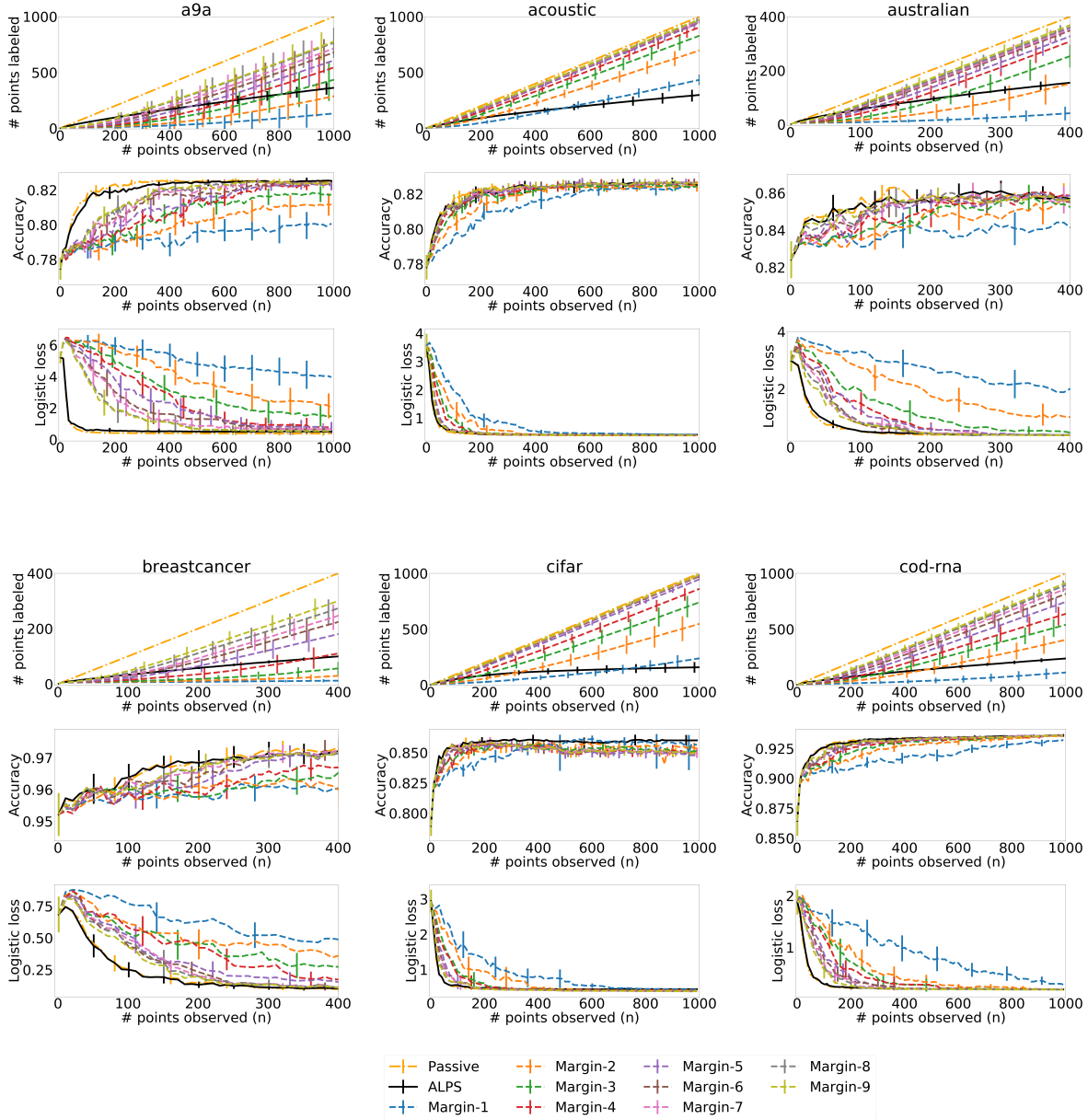
Figure 6: Comparison of all nine margin algorithms to passive learning and ALPS for 3-layer networks (1/3). The margin algorithms are ordered from the smallest to the largest threshold in \Gamma_m , where Margin-1 corresponds to the smallest threshold, Margin-2 to the second smallest, etc. The figures shows the mean over the 50 trials and twice its standard error of the number of labeled points, accuracy and logistic loss on the test set of the model returned by each algorithm as a function of the number of observed points (or rounds) n .
