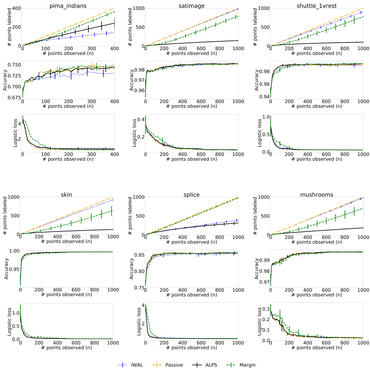
Figure 5: Comparison of the ALPS algorithm, the IWAL algorithm, the ex-post best margin algorithm and the passive learning algorithm for 3-layer networks (3/3). The figures shows the mean over the 50 trials and twice its standard error of the number of labeled points, accuracy and logistic loss on the test set of the model returned by each algorithm as a function of the number of observed points (or rounds) n .
