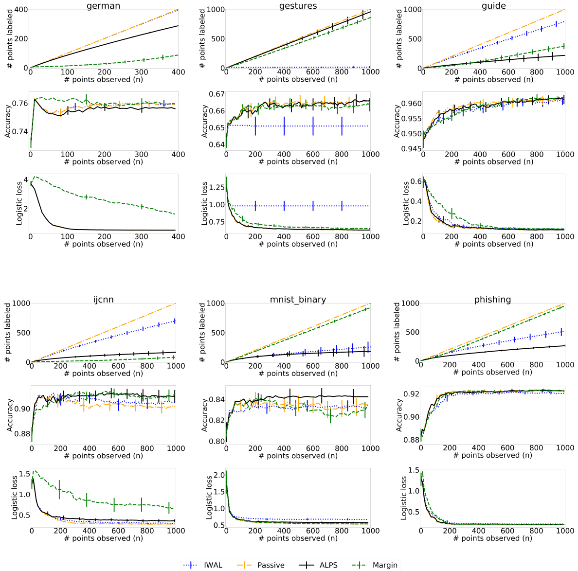
Figure 10: Comparison of the ALPS algorithm, the IWAL algorithm, the ex-post best margin algorithm and the passive learning algorithm for 4-layer networks (2/3). The figures shows the mean over the 50 trials and twice its standard error of the number of labeled points, accuracy and logistic loss on the test set of the model returned by each algorithm as a function of the number of observed points (or rounds) n .
