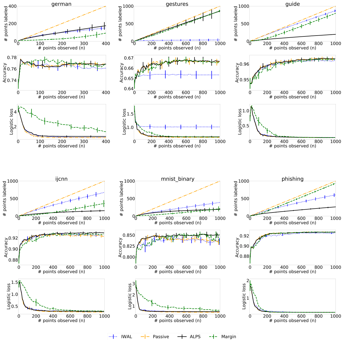
Figure 4: Comparison of the ALPS algorithm, the IWAL algorithm, the ex-post best margin algorithm and the passive learning algorithm for 3-layer networks (2/3). The figures shows the mean over the 50 trials and twice its standard error of the number of labeled points, accuracy and logistic loss on the test set of the model returned by each algorithm as a function of the number of observed points (or rounds) n .
