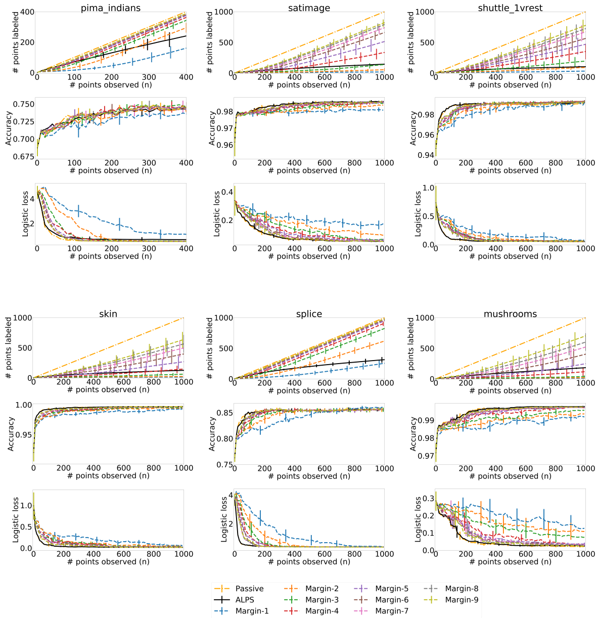
Figure 8: Comparison of all nine margin algorithms to passive learning and ALPS for 3-layer networks (3/3). The margin algorithms are ordered from the smallest to the largest threshold in \Gamma_m , where Margin-1 corresponds to the smallest threshold, Margin-2 to the second smallest, etc. The figures shows the mean over the 50 trials and twice its standard error of the number of labeled points, accuracy and logistic loss on the test set of the model returned by each algorithm as a function of the number of observed points (or rounds) n .
