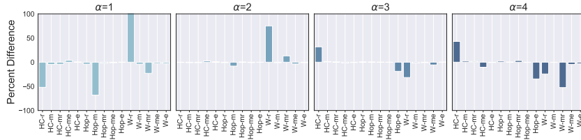
Figure 6: Percent difference of the performance of an ablation over \alpha , compared to the full algorithm. Recall the form of the sole hyperparameter \lambda = \frac{\alpha}{\sum_{(s,a)} |Q(s,a)|} , where \lambda weights the Q function during the policy update. \alpha = 2.5 is used by default. HC = HalfCheetah, Hop = Hopper, W = Walker, r = random, m = medium, mr = medium-replay, me = medium-expert, e = expert. While there is effectively no performance difference between \alpha = 2 and \alpha = 3 , we remark that performance begins to degrade on select tasks as the algorithm begins to approach more RL ( \alpha = 4 ) or imitation ( \alpha = 1 ).
