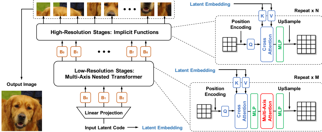
Figure 1: HiT architecture. In each stage, input the feature is first organized into blocks (denoted as B_i ). HiT’s low-resolution stages follow the decoder design of Nested Transformer [73] which is then enhanced by the proposed multi-axis blocked self-attention. We drop self-attention operations in the high-resolution stages, resulting in implicit neural functions. The model is further boosted by cross-attention modules which allow intermediate features to be modulated directly by the input latent code. The detailed algorithm can be found in the supplementary materials.
