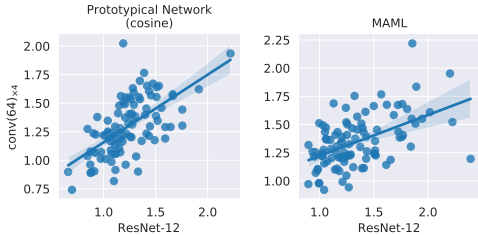
Figure 3: Episode difficulty transfers across network architectures. Scatter-plots (with regression lines) of the episode difficulty computed by \text{conv}(64)_4 and ResNet-12’s trained using different algorithms. This is computed for 10k 1-shot 5-way test episodes from Mini-ImageNet. We observe a strong positive correlation between the computed values for both network architectures.
