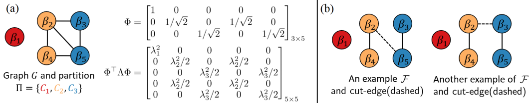
Figure 1: Illustrative example of (a) graph partition and corresponding parameters when \beta \in \mathbb{R}^5 forms K = 3 clusters, \mathcal{C}_1 = \{1\} , \mathcal{C}_2 = \{2, 4\} , \mathcal{C}_3 = \{3, 5\} ; (b) compatible forest \mathcal{F} and cut-edge(s).
