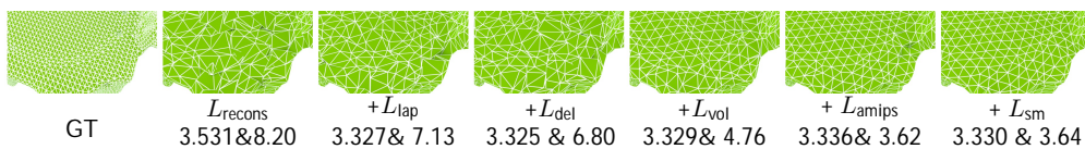
Figure 1: Ablation studies on regularization terms. We sequentially add regularizations from left to right. We show the corresponding Chamfer Distance \downarrow (CD) & AMIPS \downarrow on the bottom.
