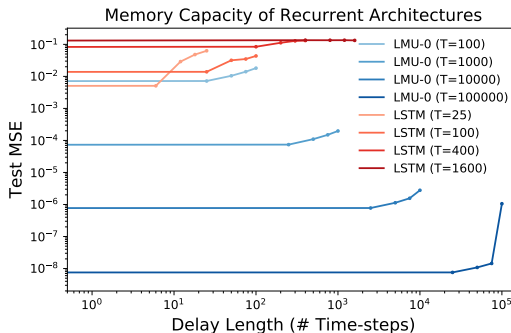
Figure 3: Comparing LSTMs to LMUs while scaling the number of time-steps between the input and output. Each curve corresponds to a model trained at a different delay window length, T , and evaluated at 5 different delay lengths across the window. The LMU successfully persists information across 10^5 time-steps using only 105 internal state-variables, and without any training. It is able to do so by maintaining a compressed representation of the 10 Hz band-limited input signal processed with a time-step of \Delta t = 1/T .
