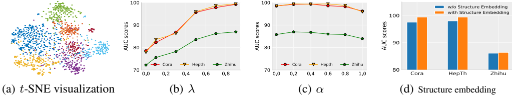
Figure 4: (a) t -SNE visualization of the learned network embedding on the CORA dataset, labels are color coded. (b, c) Sensitivity analysis of hyper-parameter \lambda and \alpha , respectively. (d) Ablation study on the use of structure embedding in the encoder. Results are reported using 95% training edges on the three datasets.
