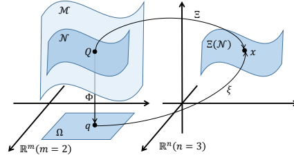
Figure 1: An illustration of manifold \mathcal{M} with local coordinate system (\mathcal{N}, \Phi) and embedding \Xi . See text for details.
