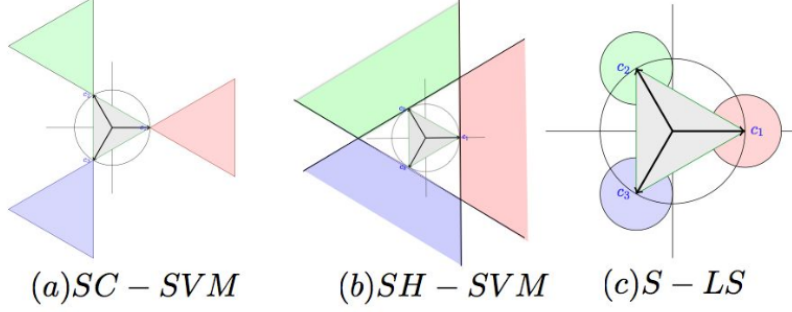
Figure 2: Level sets of the different losses considered for T = 3 . A classification is correct if an input (x, y) is mapped to a point f(x) that lies in the neighborhood of the vertex c_y . The shape of the neighborhood is defined by the loss. It takes the form of a cone supported on a vertex, in the case of SC-SVM, a half space delimited by the hyperplane orthogonal to the vertex in the case of the SH-SVM, and a sphere centered on the vertex, in the case of S-LS.
