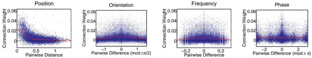
Figure 2: Connection weights versus pairwise differences of four properties of linear basis functions, estimated by fitting 2D Gabor functions. The curves were fit by local Gaussian smoothing.
