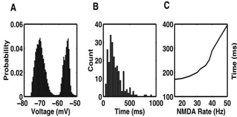
Figure 2: A. Histogram of the up and down states. B. Dwell times of the up states C. Mean duration of the up states increases with rate of NMDA inputs. Each histogram was calculated over a run of 120 seconds.
