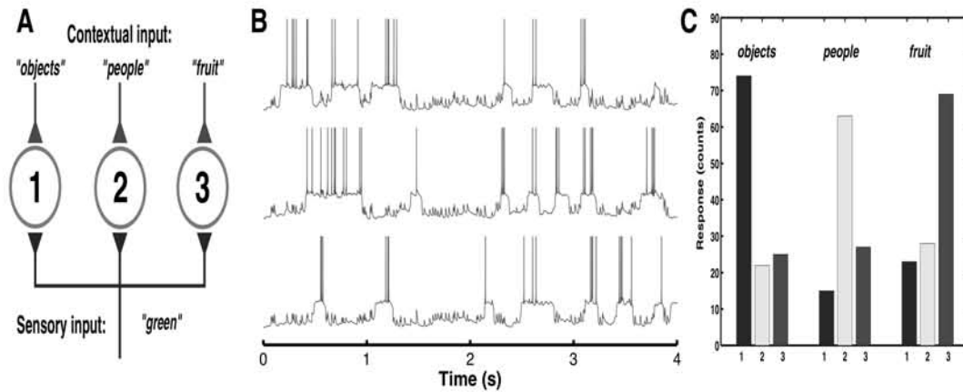
Figure 4: A. Illustrative task for contextual processing in semantic inference. 3 neurons each receive independent contextual (NMDA) and common informational (AMPA) input. B. Voltage traces showing differences in firing patterns depending upon context. C. Each neuron is tuned to its defined context. Correlation was measured between the informational spike train and each contextual spike train smoothed with a gaussian filter ( \sigma = 60ms ). The most correlated context was defined to be the right one and the spikes of all neurons were counted.
