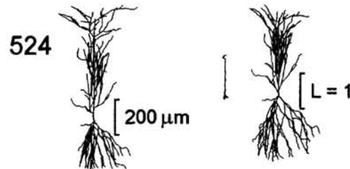
Figure 3: CA1 pyramidal cell anatomy (cell 524, left) with neuromorphic renderings of V_{out} (middle) and V_{in} (right) transforms at DC.
