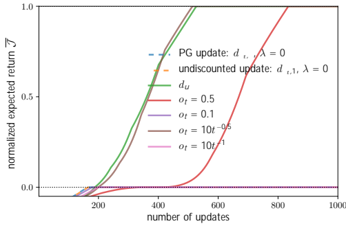
(a) vs t , with \gamma = 0.95, jSj = 10, \beta = 1
