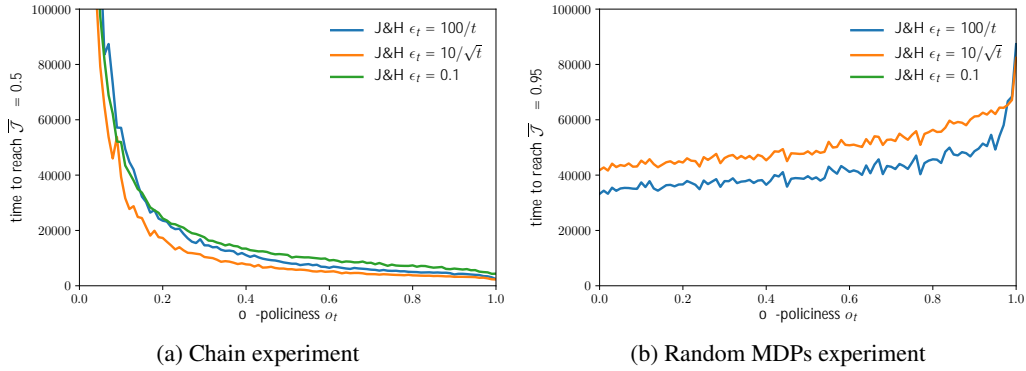
Figure 10: Experiments vs. off-policiness o_t : average time to reach a global performance objective.
