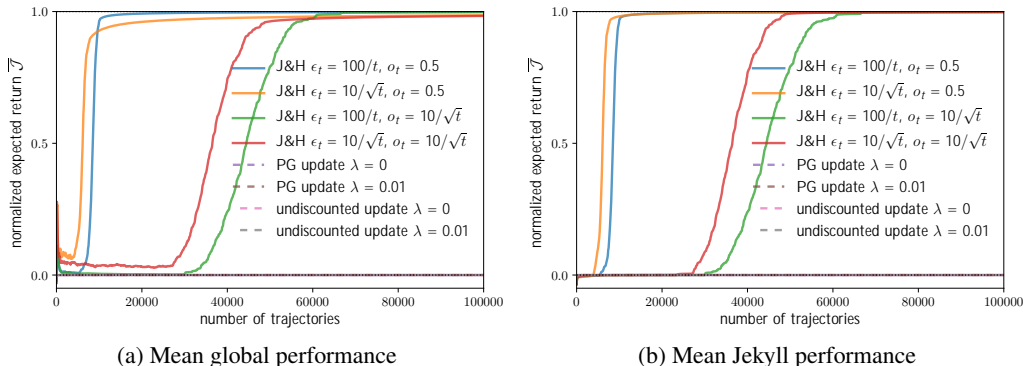
Figure 8: Chain MDPs experiments vs. number of trajectories (200+ runs).
