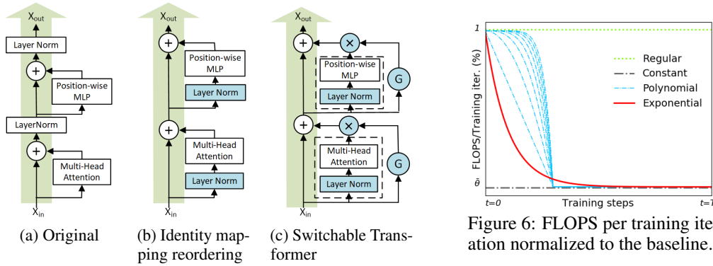
Figure 5: Transformer variants, showing a single layer block.
