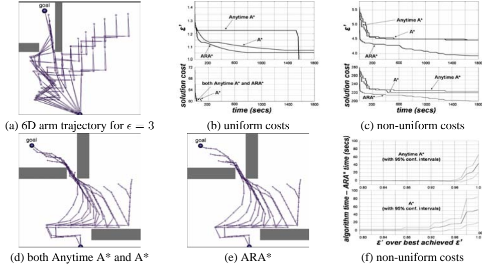
Figure 4: Top row: 6D robot arm experiments. Bottom row: 20D robot arm experiments (the trajectories shown are downsampled by 6). Anytime A* is the algorithm in [8].
