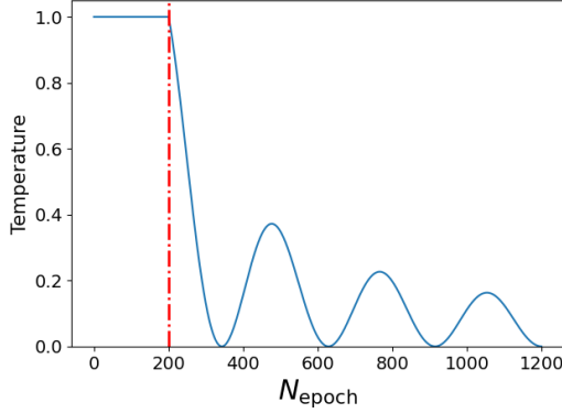
Figure 4: Illustration of the cosine modulated annealing schedule. The plot depicts the annealing schedule with N_{\text{warmup}} = 200 and N_{\text{anneal}} = 1000 steps. The vertical red line marks the end of the warmup phase.
