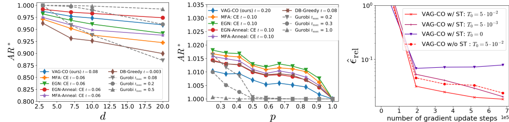
Figure 1: Left: Comparison of AR^* for the MIS problem on the RRG-100 dataset with different degrees d . Middle: Results for the MVC problem in terms of AR^* on the RB-200 dataset at different generation parameters p . Left, Middle: Values closer to one are better. The runtime t is given in s/graph and t_{\max} is the time limit for Gurobi. Right: Ablation on annealing and subgraph tokenization (ST). The \hat{\epsilon}_{rel} on the RB-100 MVC is plotted over the number of gradient update steps. Lower values are better.
