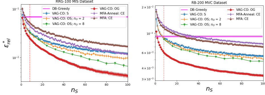
Figure 3: Ablation on different sampling strategies for VAG-CO on the RRG-100 MIS dataset (Left) and on the RB-200 MVC Dataset (Right). The averaged best relative error \epsilon_{\text{rel}}^* on the test dataset is plotted over the number of solutions n_S per graph. Error bars indicate the standard error over the test dataset.
